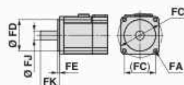
Applicable Motor dimensions
