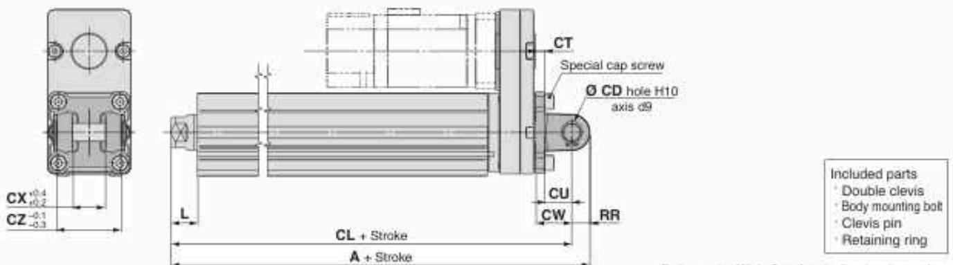
Double Clevis [mm]
