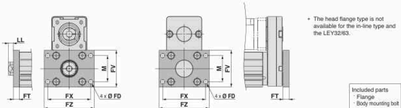
Rod/Head Flange [mm]
