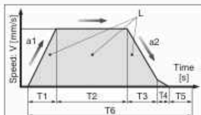
<Speed-Work Load Graph> (LET100)
